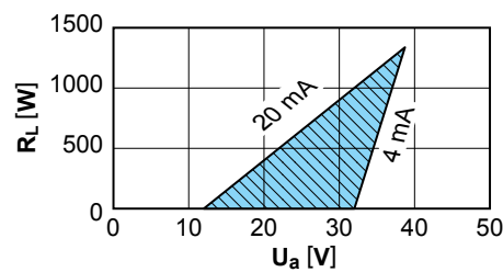
Fig.2-18 R_L = f(U_a) diagram of the LE 2XX Series Load Measuring Pins operating range
